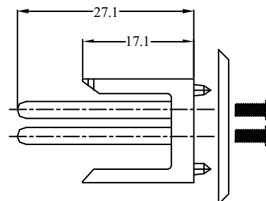
Keying Pin
